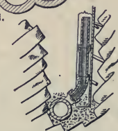
FIG. 9. DEEP-CUT HOUSE CONNECTION IN ROCK.
